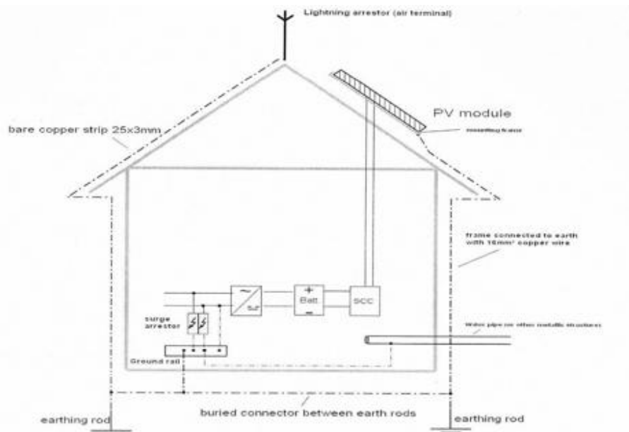
Fig. 2 Equipment bonding for grounding and lightning protection for a solar –PV site.
