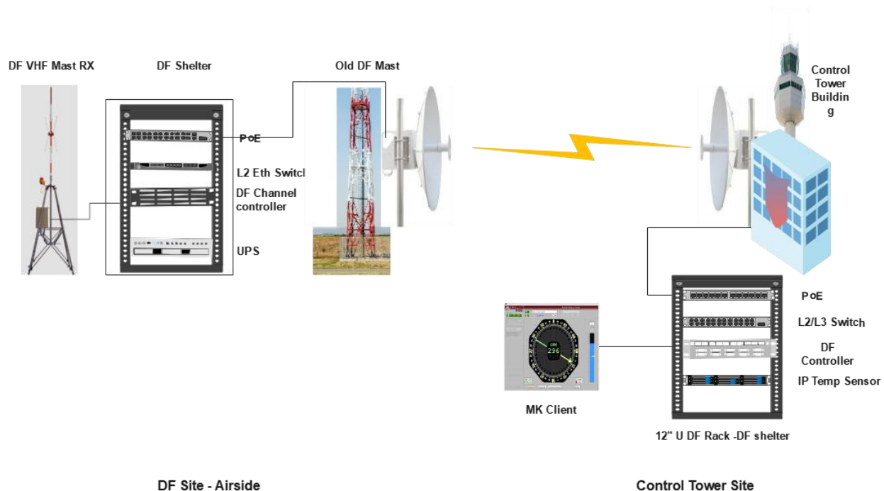
Fig. 1 Eldoret VDF Microwave Link Architecture
